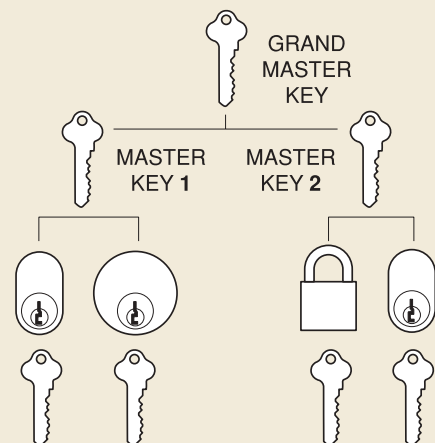
Example of a Grand Master Key System
